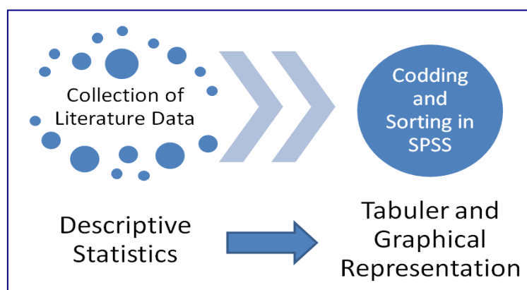
Figure 2- Analysis Framework
